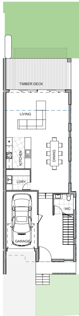
GROUND FLOOR
