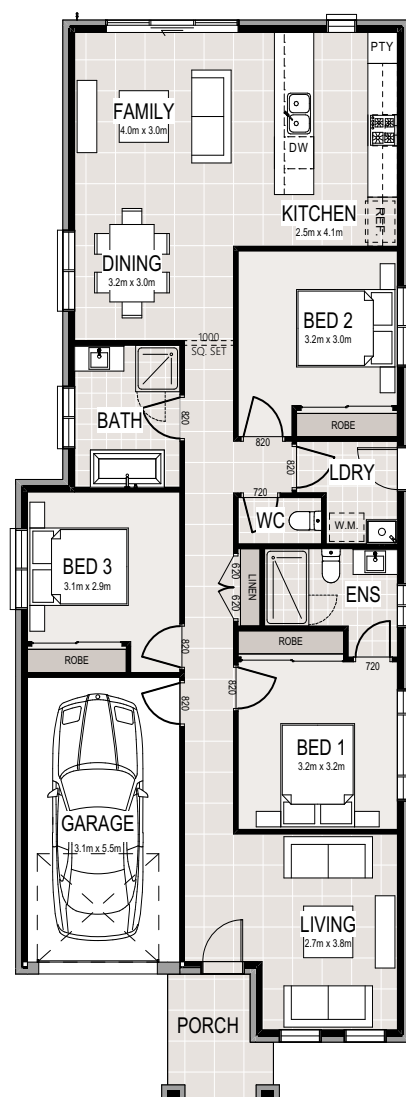
FLOOR PLAN
