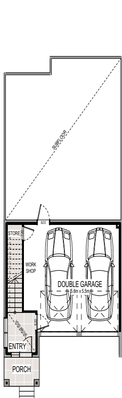
GARAGE PLAN
