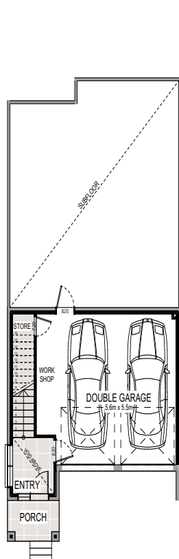
GARAGE PLAN
