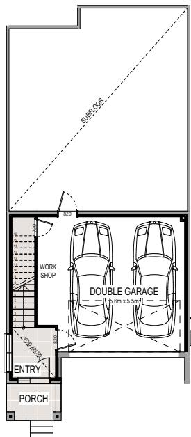
GARAGE PLAN
