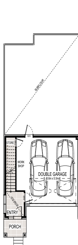
GARAGE PLAN
