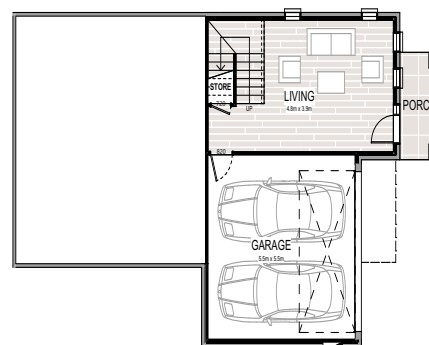
LOWER GROUND FLOOR PLAN
