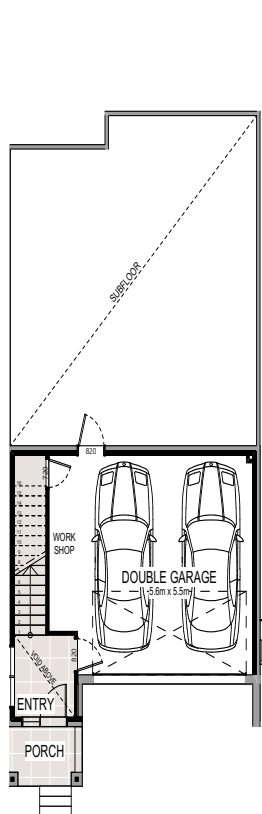
GARAGE PLAN
